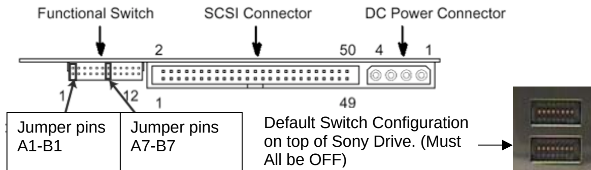
SONY SMO-F551-SD MOD DRIVE ILLUSTRATION 4-1
